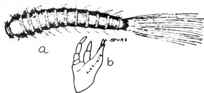
Fig. 244. a, Carpet beetle; b, Maxilla.
